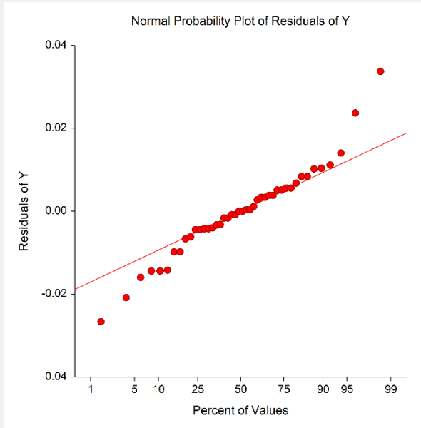
Probability Plot of Residuals
